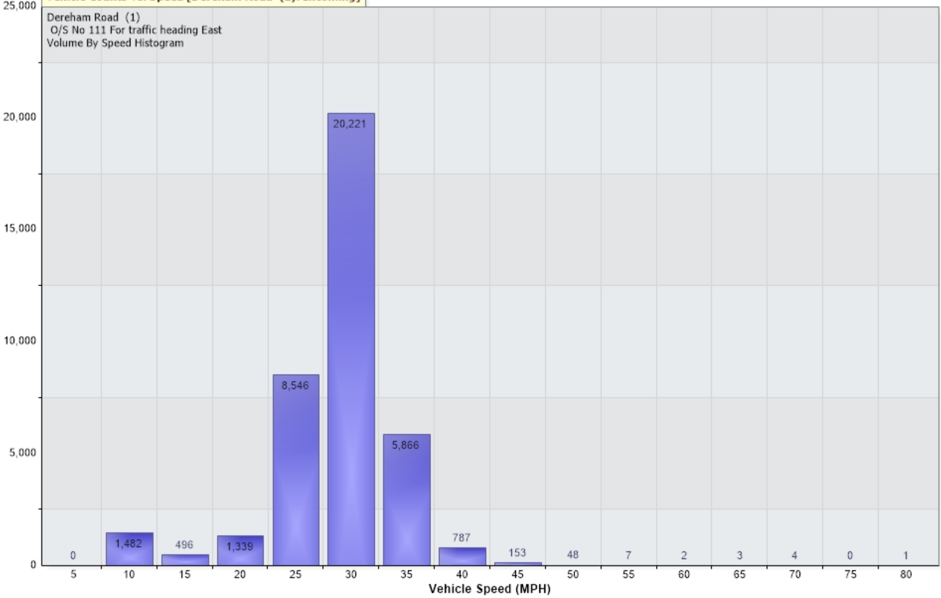
Vehicle Counts Vs. Speed [Dereham Road (1): Incoming]
