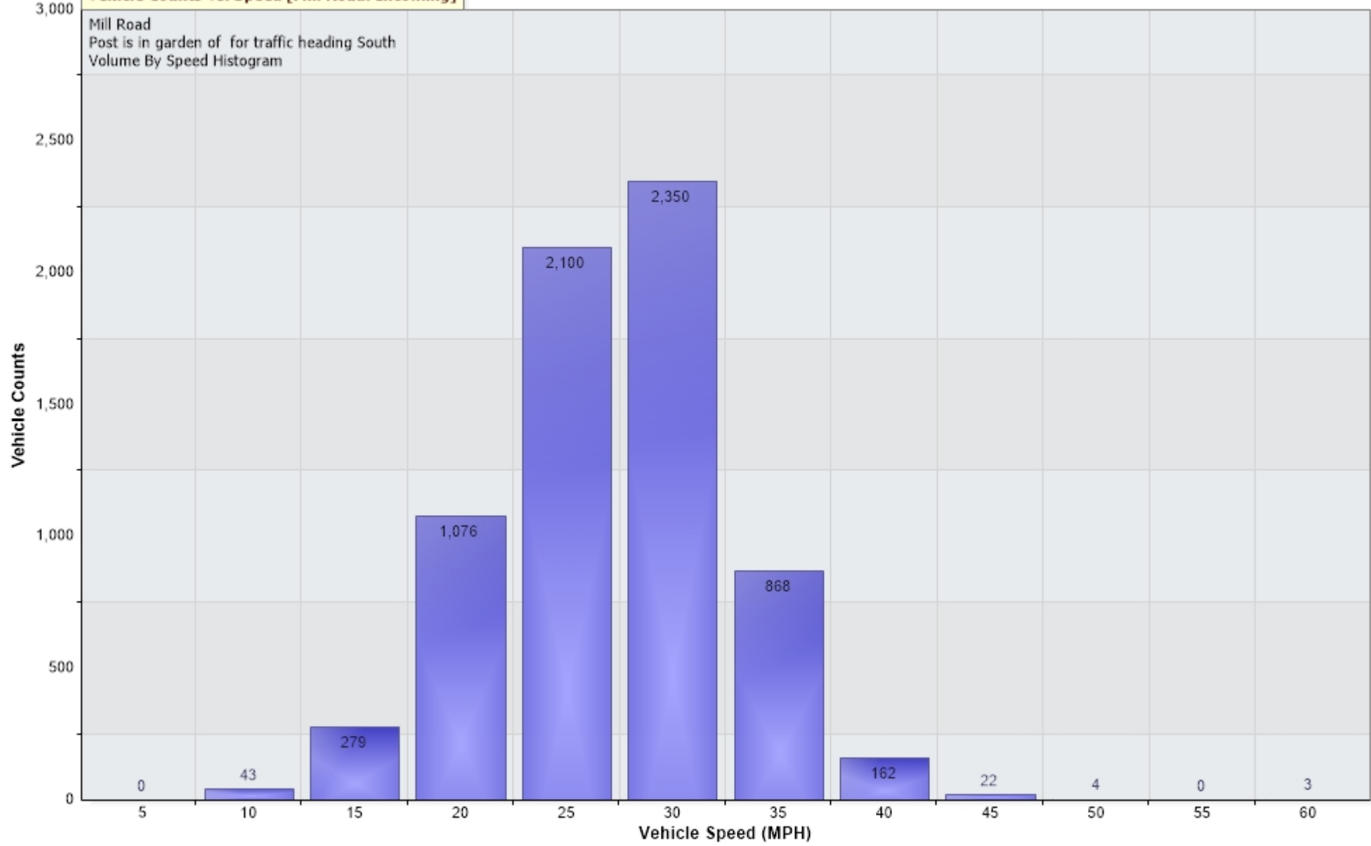
Vehicle Counts Vs. Speed [Mill Road: Incoming]
