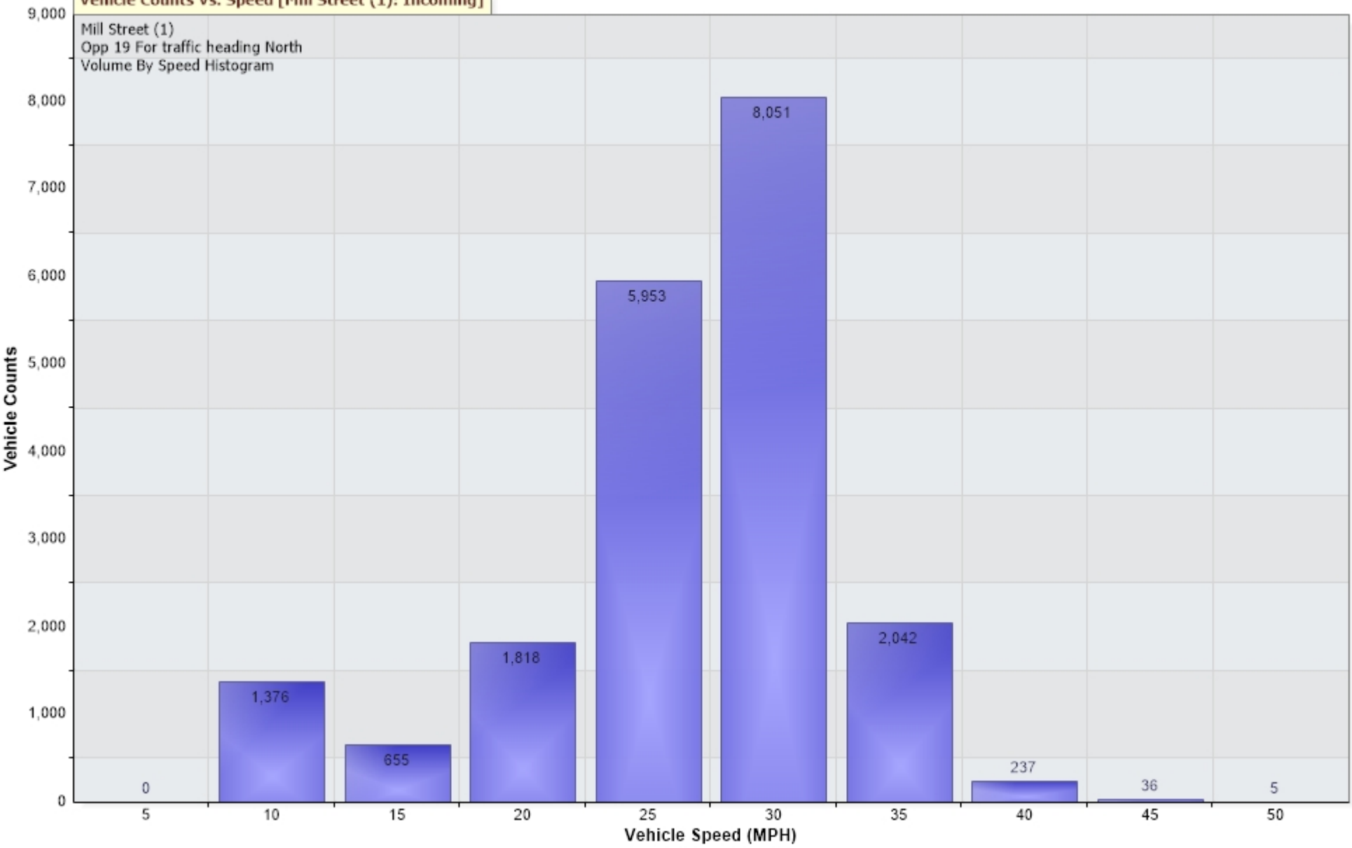
Vehicle Counts Vs. Speed [Mill Street (1): Incoming]
