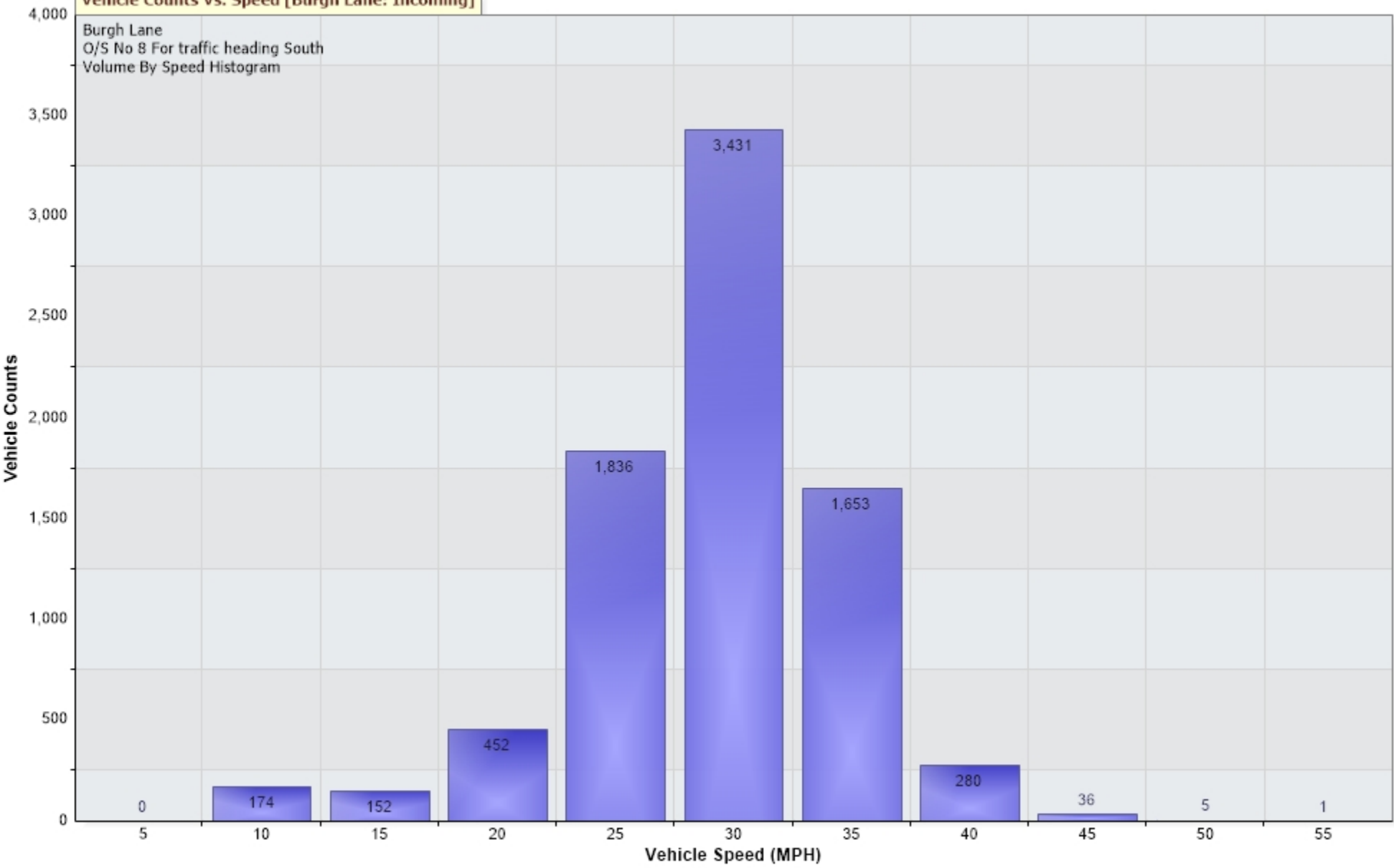
Vehicle Counts Vs. Speed [Burgh Lane: Incoming]
